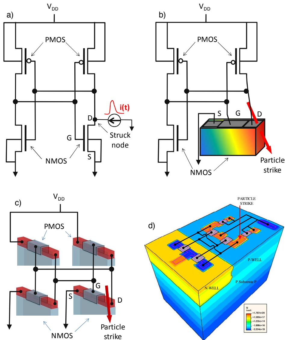
Fig. 30. Illustration of the simulation methods that can be used to investigate single-event effects at circuit level (here illustrated for a SRAM cell): (a) SPICE simulation; (b) mixed-mode simulation; (c) numerical simulation with several discontinuous domains connected using a mixed-mode approach; (d) full 3-D numerical simulation with one continuous domain. The snapshot of the full 3-D 6T SRAM cell (d) is courtesy from P. Roche (STMicroelectronics) [80].
