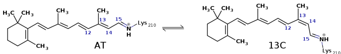
Figure 1: AT and 13C conformations of the retinal chromophore in ASR. Retinal is bound to the opsin through a protonated Schiff base with the Lysine 210 residue. The photoinduced isomerization involves the dihedral angle defined by carbon atoms 12, 13, 14, and 15.
