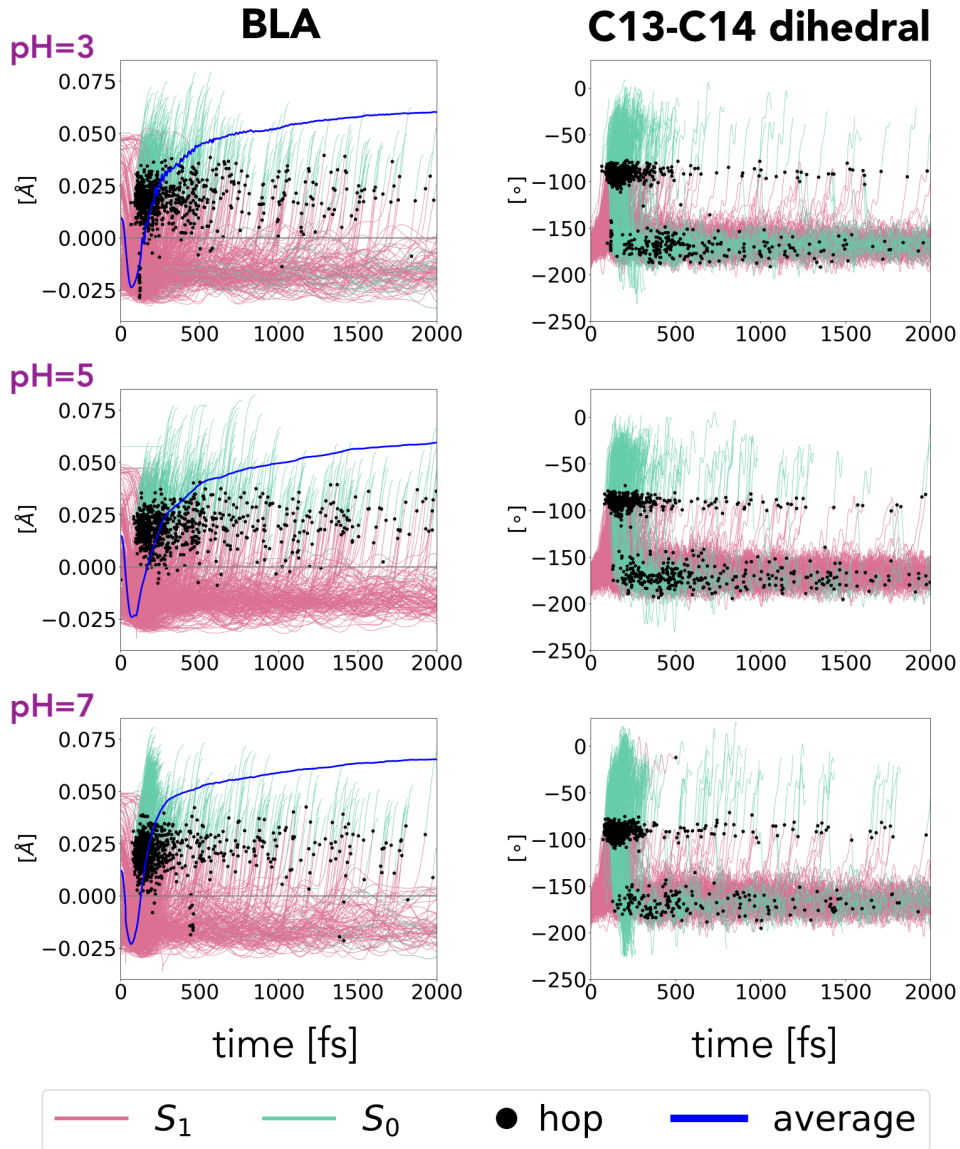
Figure 3: Time evolution of BLA (left) and torsion dihedral angle (right) during the AT \rightarrow 13C retinal isomerization. S_1 (pink) and S_0 (green) parts of a trajectory are separated by a hop point (black circle). The BLA instantaneous average values are also plotted in blue. Please note that, since the trajectories are stopped shortly after reaching S_0 , their last BLA value is frozen for the remainder of the averaging to avoid noise and discontinuities.
