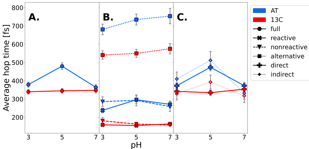
Figure 6: S_1 \rightarrow S_0 \bar{t}_{\text{hop}} as a function of pH for AT and 13C models; standard errors are given as grey error bars. (A) Full set of valid trajectories. (B) Reactive, nonreactive, alternative channels. (C) Direct and indirect subsets.
