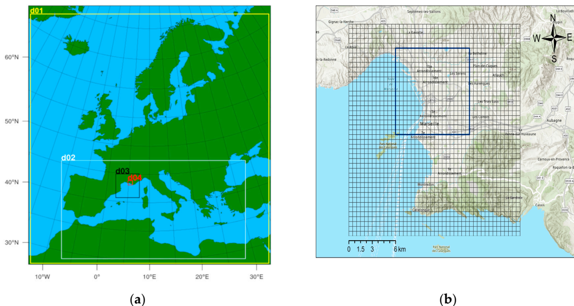
Figure 1. Maps of computational domains of the coupled CTM setup for Marseille simulations: (a) nested domains for CMAQ simulations over Europe with horizontal grid resolutions 36 \text{ km} \times 36 \text{ km} (yellow frame, d01), 12 \text{ km} \times 12 \text{ km} (white frame, d02), and 4 \text{ km} \times 4 \text{ km} (black frame, d03); (b) urban domain for EPISODE-CityChem simulations with extent of 22 \text{ km} \times 22 \text{ km} and grid resolution of 500 \text{ m} \times 500 \text{ m} (zoom into area indicated by red frame, d04, in figure part (a)). Dark blue frame in figure part (b) indicates the extent of the port city area.
