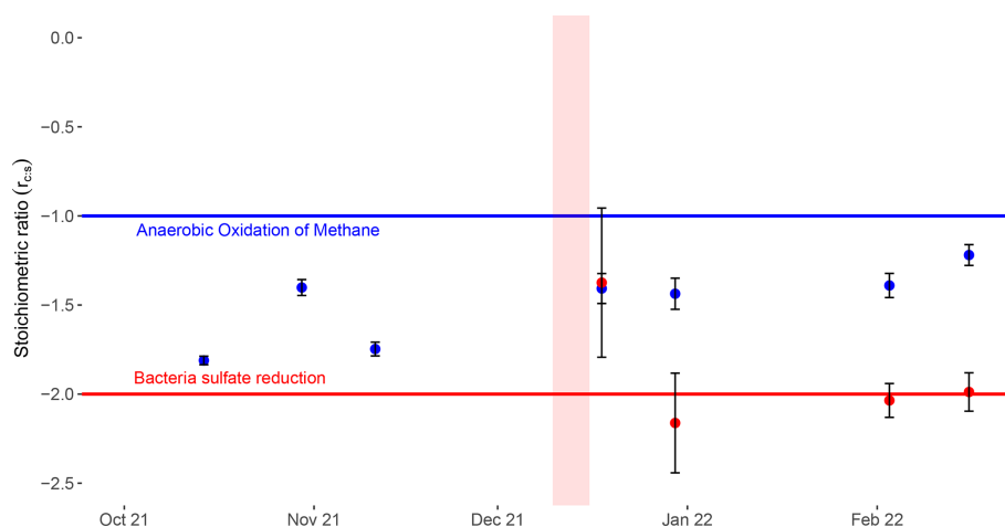
Figure 8. Temporal variation in \text{DIC} : \text{SO}_4^{2-} porewater ratio ( r_{c,s} ) calculated at the surface or at the depth of the sediment layer. The red bar indicates the flood period; before the flood the entire core is considered to be like the surface layer. Red dots represent the surface sediment layer (flood layer < 25 cm), and blue dots represent the bottom sediment layer (former sediment). The blue line indicates the theoretical stoichiometric ratio of the anaerobic oxidation of methane (−1), and the red line indicates the theoretical stoichiometric ratio of the sulfate reduction (−2).
