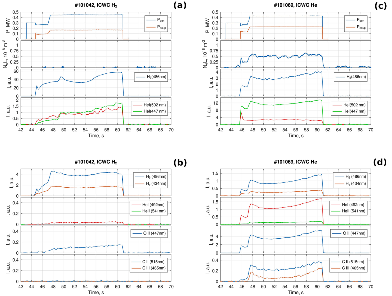
Fig. 4. (a, c) Time evolutions of generated P_{gen} and coupled P_{coup} powers, line integrated electron density N_e L (LID 3, see Fig. 1 a), optical emission intensities of H I and He I (horizontal midplane, KS 3, see Fig. 1 b). (b, d) Time evolutions of optical emission intensities of H I, He I and He II, O II, C II, C III (vertical, inner divertor, KS 3 see Fig. 1 b). The ICWC discharge in H _2 (left), the ICWC discharge in He (right).
