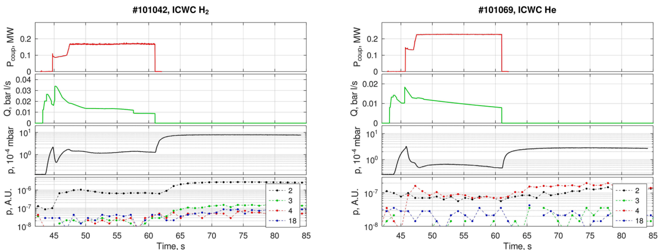
Fig. 6. Time evolutions of coupled power P_{coupl} , gas flow rate Q , pressure p , mass spectrum. The ICWC discharge in H_2 (left), the ICWC discharge in He (right).
