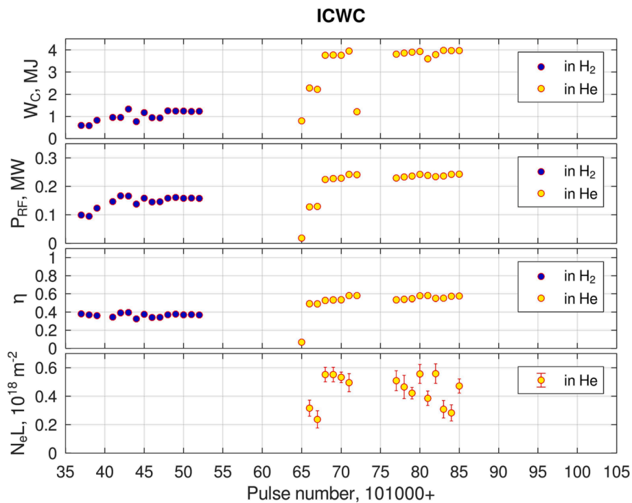
Fig. 5. The total coupled energy W_c , the average value at the time interval 50–55 s coupled power P_{coupl} , coupling efficiency \eta , line integrated electron density N_{eL} (LID 3, see Fig. 1a).
