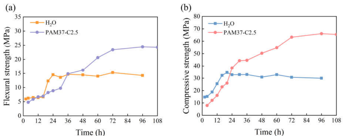
Figure 7. Variation curves of (a) flexural strength and (b) compressive strength over reaction time for hydration-hardening specimens of \alpha -HHG/PAM37-C2.5 composite material and \alpha -HHG/H 2 O.
