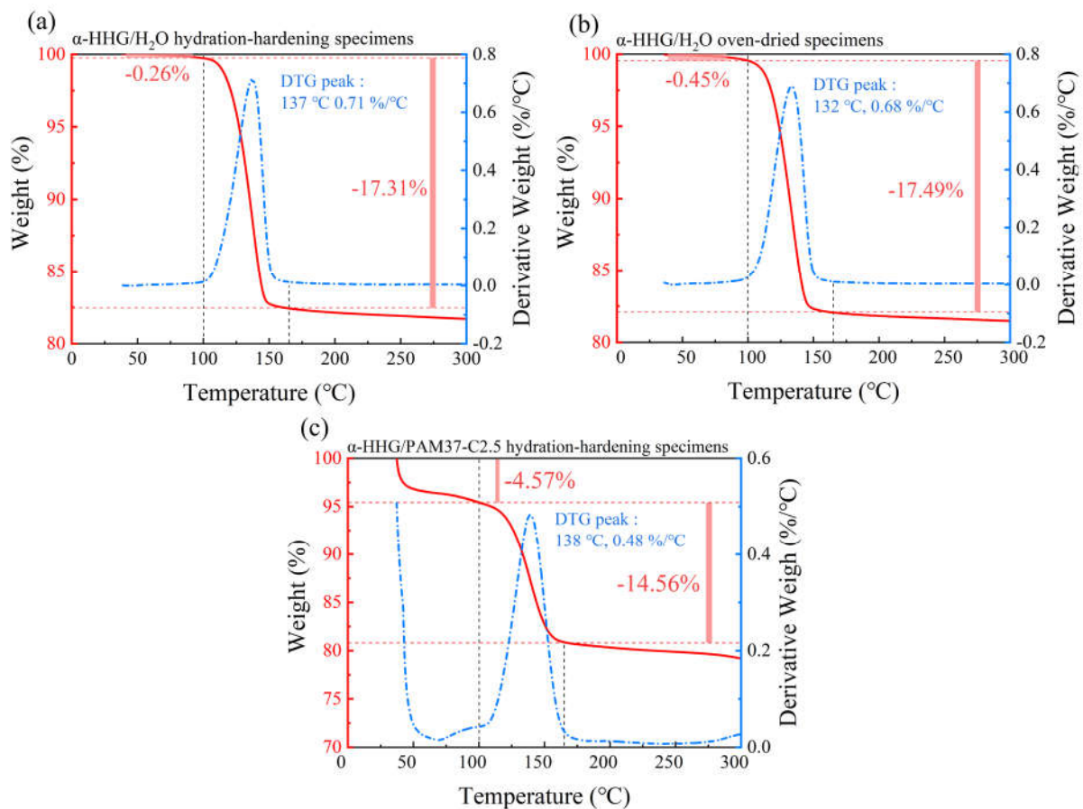
Figure 6. Thermogravimetric analysis (TGA) curves for (a) hydration-hardening specimens of \alpha -HHG/H 2 O, (b) oven-dried specimens of \alpha -HHG/H 2 O, and (c) hydration-hardening specimens of \alpha -HHG/PAM37-C2.5 composite material. The red curve illustrates the proportion of sample mass change with temperature, while the blue curve indicates the dependency of the rate of mass change on temperature, obtained through differentiation of the TGA curve.
