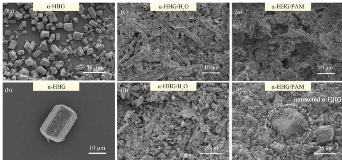
Figure 5. FE-SEM images of (a,b) raw \alpha -HHG, (c,d) oven-dried specimen fractures of \alpha -HHG/ \text{H}_2\text{O} , and (e,f) oven-dried specimen fractures of \alpha -HHG/PAM37-C2.5 composite material.
