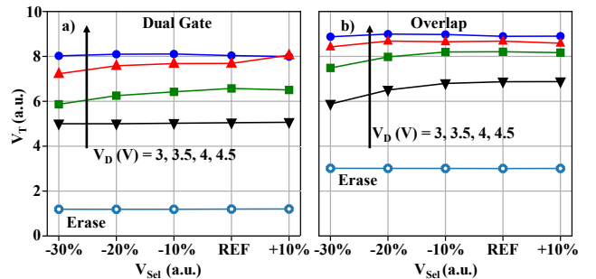
Fig. 5. SONOS eSTM™ program threshold voltage ( V_T ) evolution versus V_{Sel} bias at various V_D for dual gate (a) and overlap (b)
