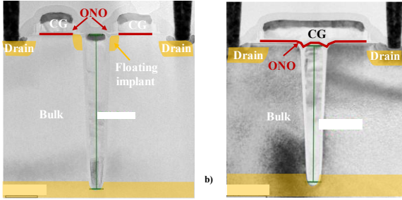
Fig. 3. SONOS eSTM™ TEM cross sections: (a) dual gate and (b) Overlap cells.
