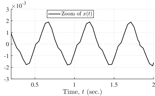
Fig. 2. Illustration of Zoom on the steady state x .
