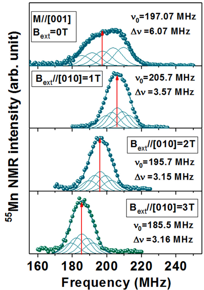
Fig. 5. ^{55}\text{Mn} NMR spectra ( \text{Mn}_I sublattice) recorded from the \text{Mn}_5(\text{Ge}_{0.6}\text{Si}_{0.4})_3 film in the external in-plane field varying between 0 and 3 T.
