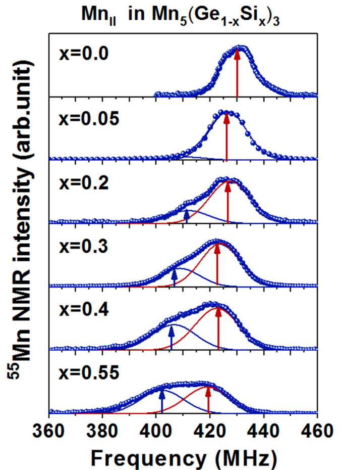
Fig. 7. Zero-field ^{55}\text{Mn} NMR spectra recorded from the Mn_{II} sublattice in a series of Mn_5(\text{Ge}_{1-x}\text{Si}_x)_3 epitaxial films ( 0 \leq x \leq 0.55 ). Red arrows indicate the NMR frequency of the original Mn_{II} line and blue arrows - the satellite line originating from the modified Mn_{II} environments.
