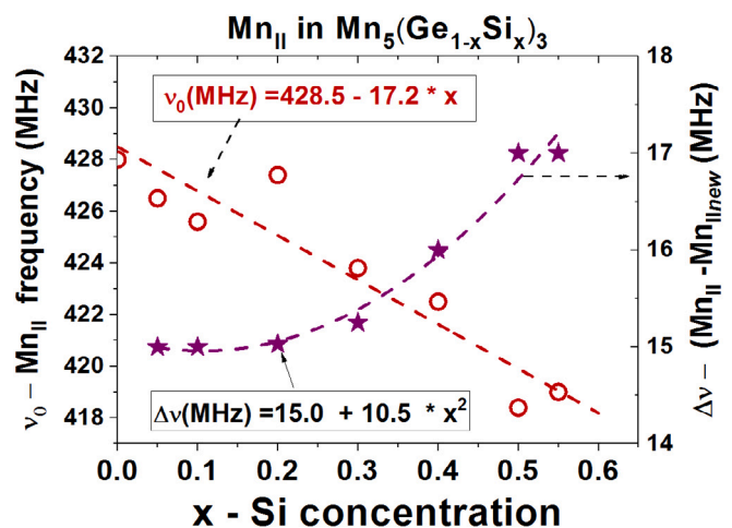
Fig. 8. ^{55}\text{Mn} NMR in the Mn_{II} sublattice as a function of Si concentration. Red open circles-NMR frequency of the original Mn_{II} line; purple stars: frequency separation between the Mn_{II} and Mn_{IInew} NMR lines.
