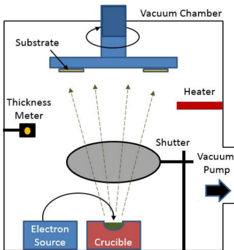
Figure 10. Simplified Electron beam evaporation system diagram.
