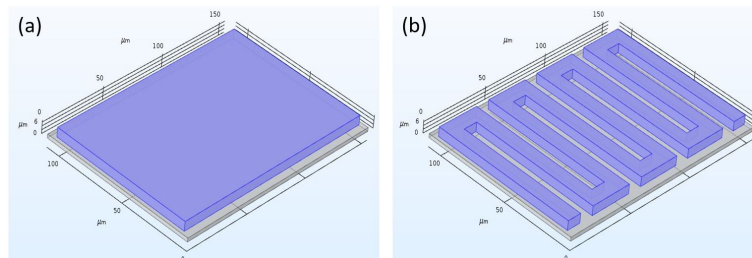
Figure 2. Thermistor shapes (a) Rectangular; (b) Serpentine.
