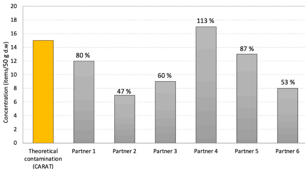
Fig. 5. Recovery rates of microplastic fragments of size class 500–1000 µm found by each partner in positive control PC2 (spiked concentration in items/50 g d.w of sediments).
