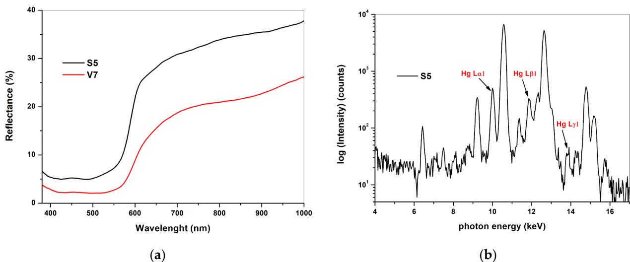
Figure 10. (a) Fiber Optics Reflectance Spectroscopy (FORS) spectra measured in area S5 (black curve) of the Mystic Marriage of Saint Catherine painting and area V7 (red curve) of the Madonna of the Rose Garden painting. The FORS spectra suggest the presence of cinnabar or vermillion, probably used together with an organic pigment, in area S5, and an iron-based pigment in area V7. (b) A detail of the ED-XRF spectrum measured in area S5 of the Mystic Marriage of Saint Catherine painting. The peaks relative to the L α1 , L β1 and L γ1 lines of mercury (Hg) are indicated.
