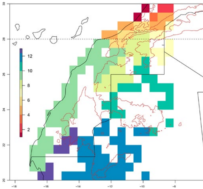
Fig. 12. – Spatial clustering of the Atlantic Sahara and neighboring areas based on the 13 bioclimatic variables.
