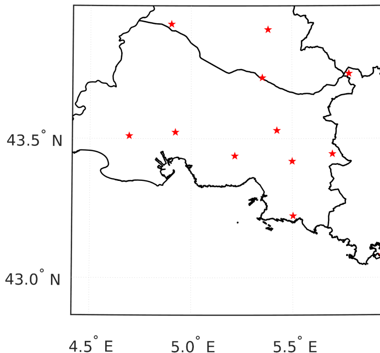
Figure A1. Positions of the twelve stations recording meteorological measurements that were within our 1 km domain boundaries.
