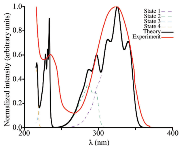
Figure 2. UV-absorption of Iso-CF 3 (red curve). The total vibrationaly resolved theoretical spectrum (black solid curve) is decomposed in the contribution for each electronic excited state (dashed lines). [32]
