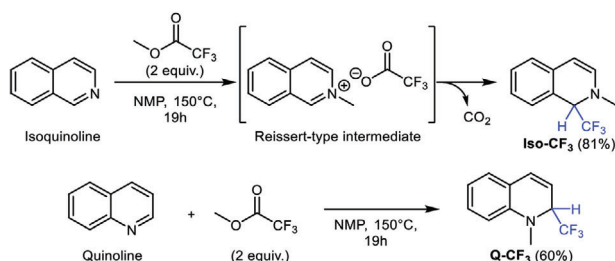
Scheme 2. Synthesis of \alpha -trifluoromethylated quinoline derivatives (NMP = N -Methyl-2-pyrrolidone).
