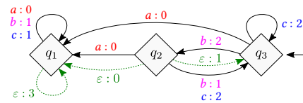
Figure 1: Automaton \mathcal{A} recognising W = \text{Inf}(a) \cup (\text{No}(a) \wedge \text{Fin}(bb)) . Many \varepsilon -transitions can be added to \mathcal{A} , some of them are depicted in dotted green.
