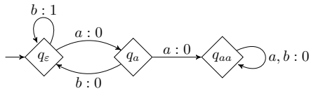
Figure 3: Büchi automaton recognising the objective W = \text{Inf}(a) \cup \text{Reach}(aa) .
