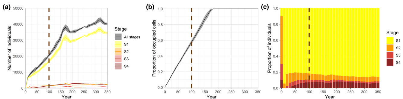
FIGURE 2 Temporal dynamics and composition of a Ligustrum lucidum population during range expansion (number of replicates = 6) S1 = saplings, S2 = small trees, S3 = medium trees and S4 = big trees. (a) Mean number \pm SE of individuals (S1–S4) over time; (b) Mean proportion \pm SE of occupied cells in the landscape over time; (c) Mean proportion of the different stages over time. The vertical dashed line represents the initial population composition used to run the experiments.
