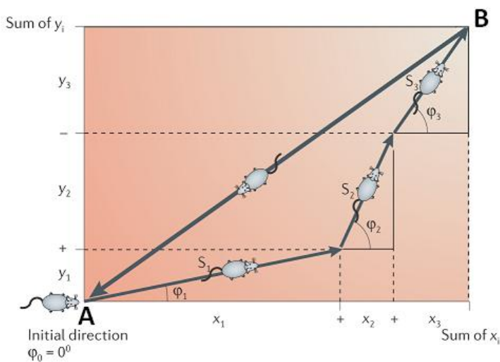
Fig. 21: Path integration.
