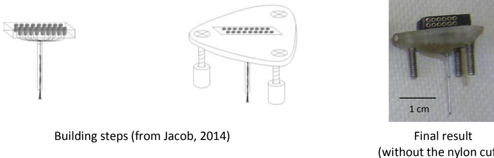
Fig. 81: Microdrive building.
