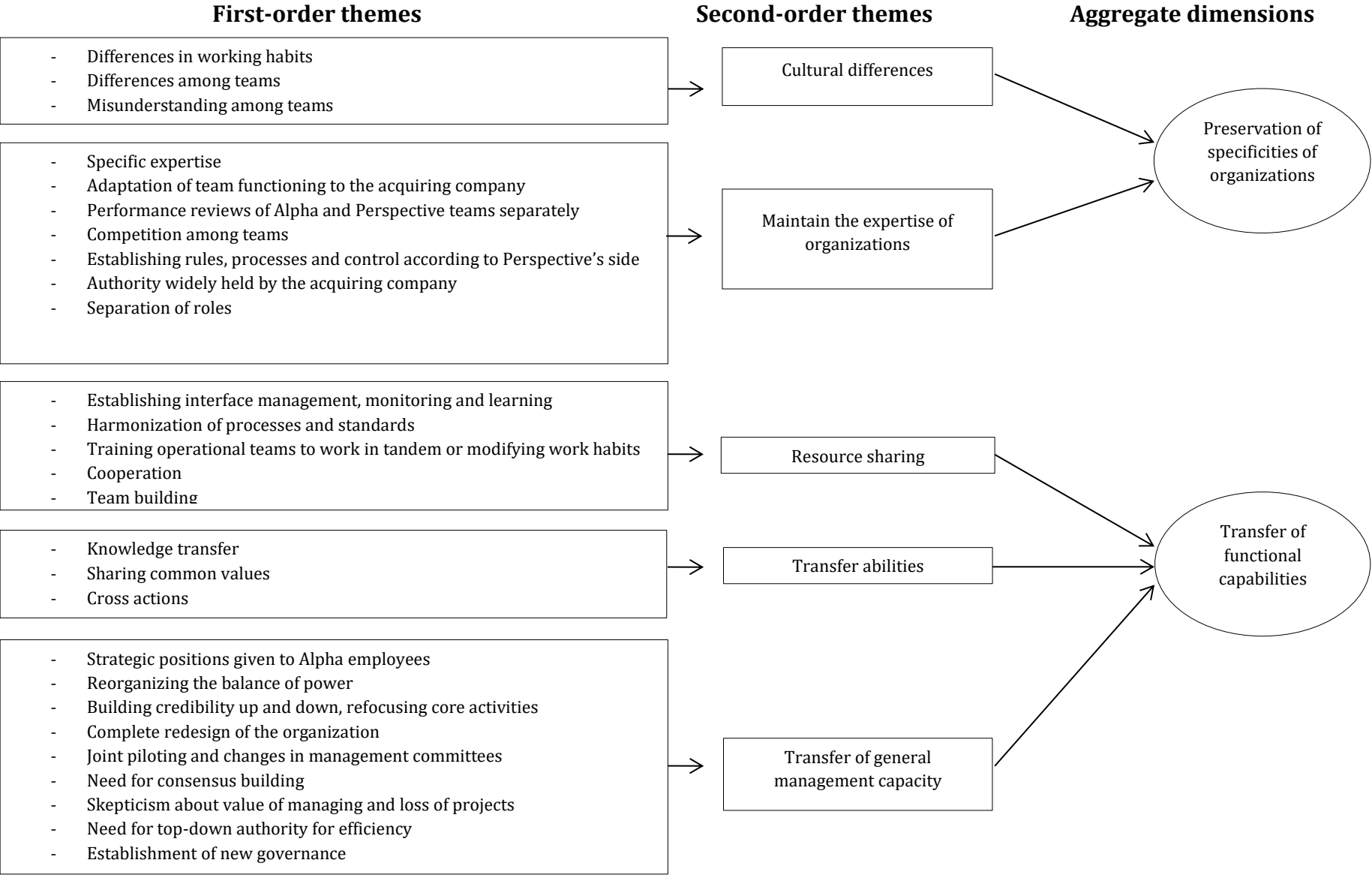
Figure 7. Data structure
