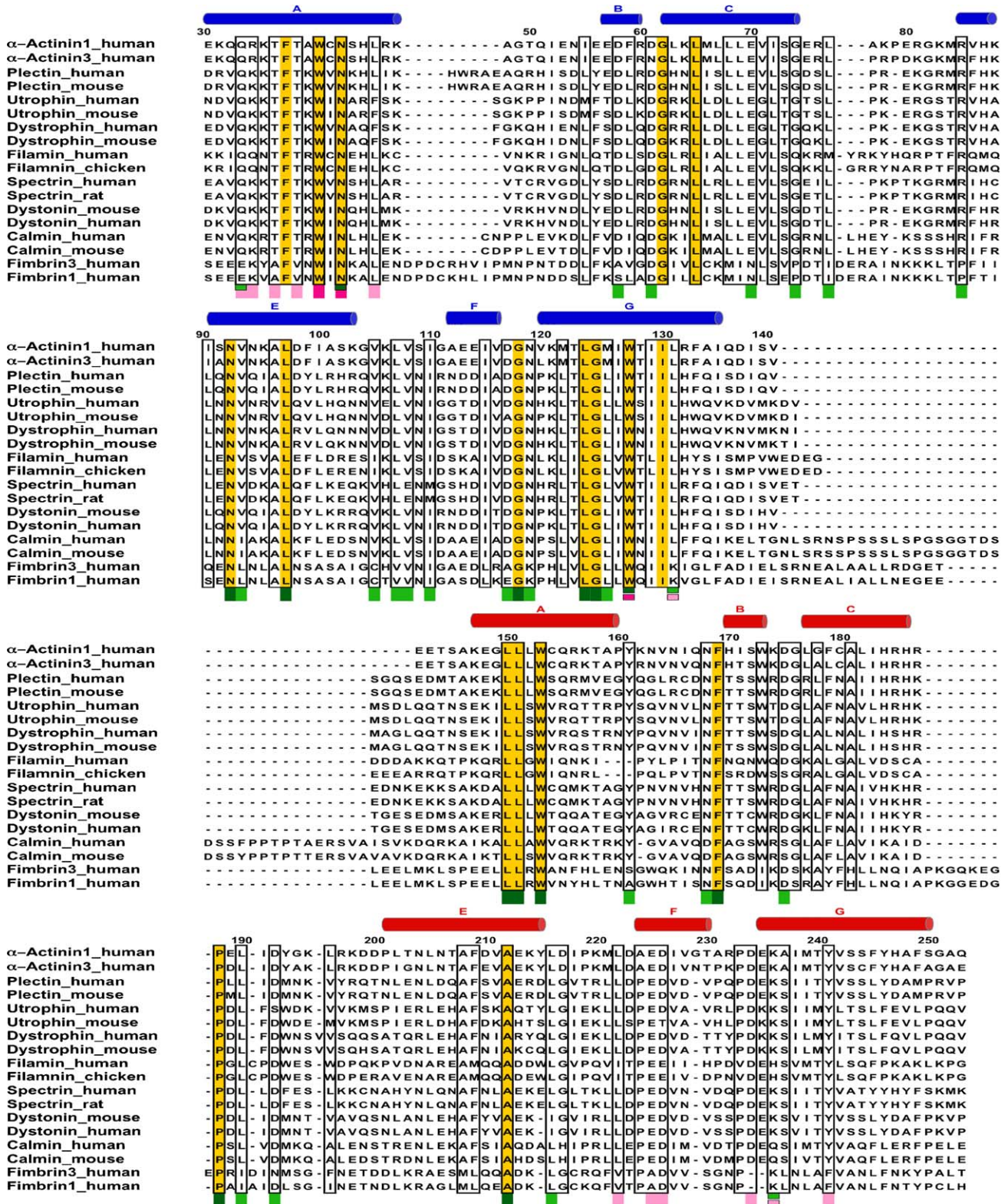
Fig. 1. Alignment of 18 representative sequences of ABD domains. Accession codes are (from top to bottom): human \alpha -actinin 1, P12814; human \alpha -actinin 3, Q08043; human plectin, G02520; mouse plectin, Q9QXS1; human utrophin, P46939; mouse utrophin (NP_035812), human dystrophin, P11532; mouse dystrophin, P11531; human filamin, O75369; chicken filamin, NP_989905; human \beta -spectrin, O15020; rat \beta -spectrin, Q9QWN8; mouse dystonin, NP_598594; human dystonin, Q03001; human calmin, Q961Q2; mouse calmin, Q8C5W0; human fimbrin (plastin 3, ABD1), BAD96521; and human fimbrin (plastin 1, ABD1), AAH31083. Invariant residues are highlighted in yellow, while residues with greater than 70% conservation are boxed. The helices of CH1 and CH2, defined according to the structure of the ABD of \alpha -actinin 1, are represented as blue and red cylinders. Residues numbers correspond to human \alpha -actinin 1. Conserved and exposed amino acids are indicated below the alignment by dark-green (100% conservation) and light-green (>70% conservation) rectangles. Similarly, conserved amino acids at the interface of the two CHs are indicated by purple (>75% conservation) and magenta (>50% conservation) rectangles.
