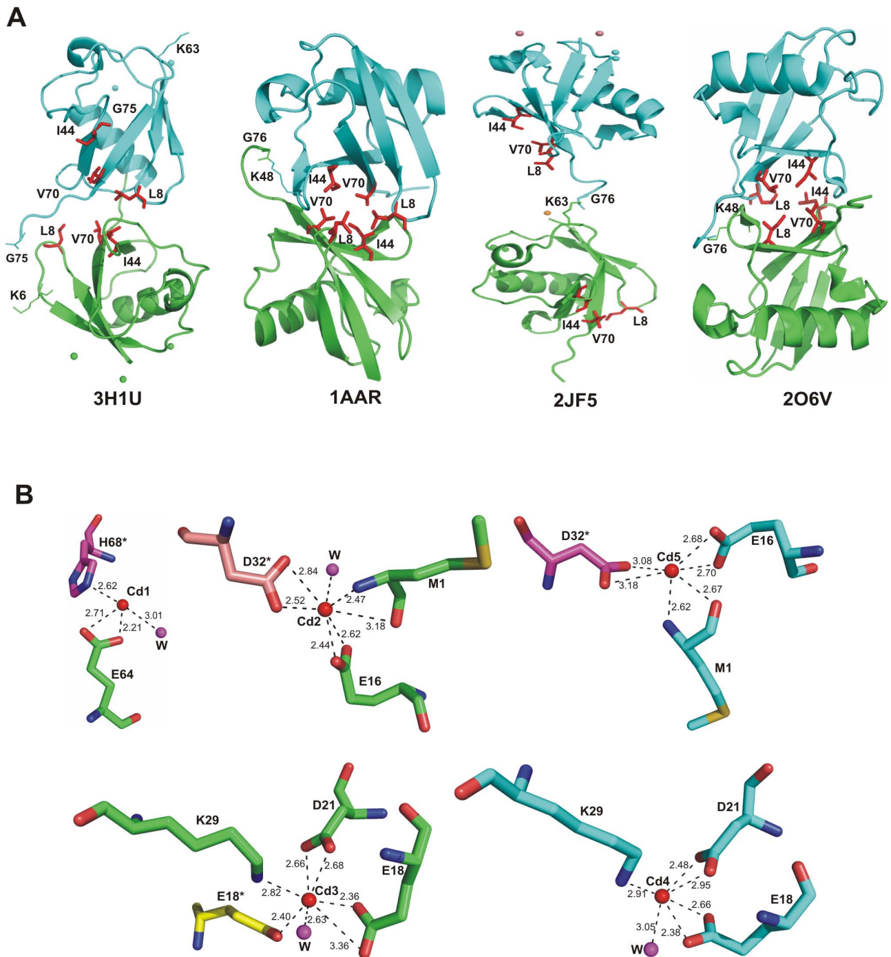
Figure 3 The hydrophobic patch and binding of cadmium ions. A. Mapping the locations of the residues that form the hydrophobic patch (Leu-8, Ile-44, and Val-70) with respect to the crystallographic dimer interface in four Ub crystal structures. Chain A are shown in green and chain B in cyan. Residues from the hydrophobic patch are shown as red sticks and labelled. When present, cadmium ions are shown as either green or cyan spheres, according to the Ub monomer they bind to. B. The five cadmium binding sites observed. Residues of chain A are in green while symmetry related molecules are shown in different colours. Contacts between cadmium ions (red spheres) and water molecules (magenta spheres) are indicated by dashed lines, with the corresponding distances labelled in Å. Oxygen atoms are coloured in red and nitrogen atoms in blue.
