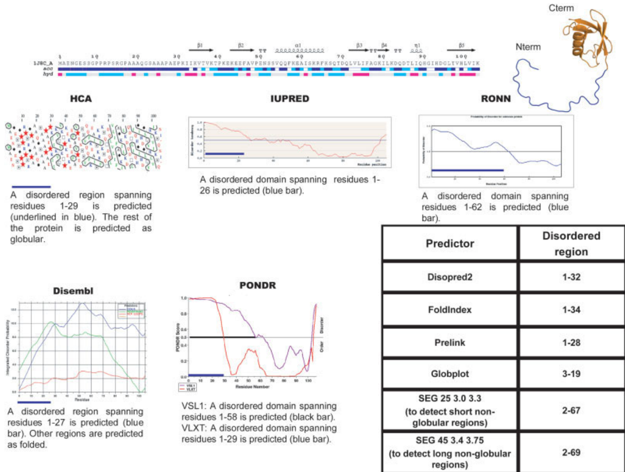
Fig. 5. Analysis of the Ubiquitin-like protein domain of hPLIC-2 (accession number: Q9UHD9) using different predictors. The protein sequence, with the secondary structure elements derived from the structure (PDB code 1J8C), is shown. The solvent accessibility of each residue is plotted below the sequence. The ribbon representation of the structure is shown; the globular domain is colored in gold while the disordered region is in blue. The picture was obtained using Pymol. The graphical output of various prediction methods and the corresponding interpretation are shown. The precise boundaries of ordered and disordered regions were derived from the corresponding text output (not shown). A blue bar highlights the disordered region for each graphical output, except for VSL1 for which the disordered region is highlighted with a black line. [Color figure can be viewed in the online issue, which is available at www.interscience.wiley.com .]
