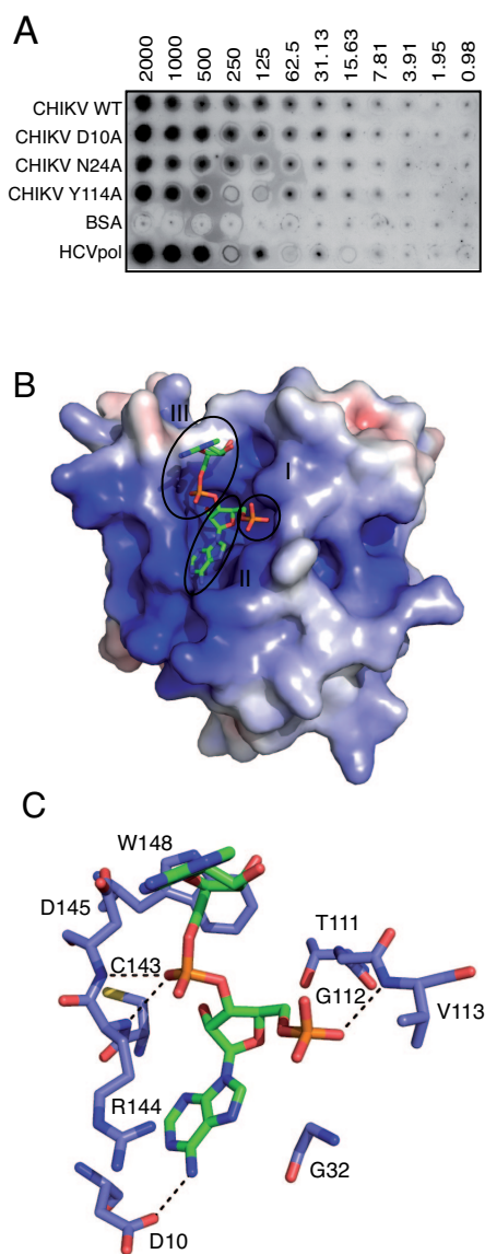
FIG. 6. RNA binding assays. (A) Slot blot RNA binding assay with wild-type and mutant CHIKV macro domains using the 5' - ^{32}\text{P} -labeled RNA AAAAAAAAAAGCUACC as a probe to label immobilized proteins. The amount of proteins blotted onto the membrane ranges from 2,000 to 0.98 pmol, as indicated. (B) Surface representation of the CHIKV macro domain in complex with the RNA AAA. Proposed nt 1, 2, and 3 (I, II, and III, respectively) are circled. The electrostatic potential is shown between -6 and 6 kT/e and has been generated as in Fig. 1C. (C) RNA binding site. RNA is shown in green and interacting residues in blue, with oxygens in red. H-bonds are indicated with dotted lines.
