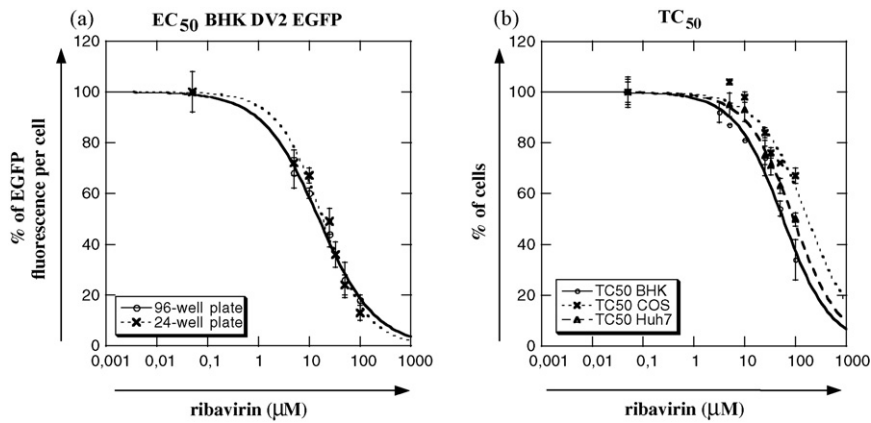
Fig. 4. Measurement of CC_{50} and EC_{50} values of ribavirin on DV EGFP-replicon cells. (a) Ribavirin EC_{50} values were calculated on BHK DV2 EGFP-replicon containing cells, from plate-carrying fluorimeter measurements (o, solid line) or obtained from flow cytometry measurements (x, dotted line). (b) From plate-carrying fluorimeter measurements, ribavirin CC_{50} values were calculated on BHK cells (solid line), COS cells (large dotted line) and Huh7 cells (thin dotted line).
