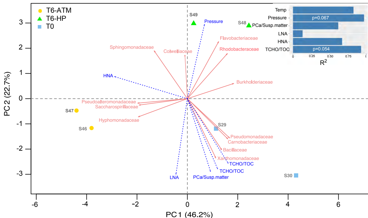
Figure 4-5 Principal Component Analysis (PCA) biplot of samples and the most contributing taxonomic families (based on fviz_contrib function of factoextra). Samples are indicated as yellow circles (ATM), green triangles (HP) or blue squares (T0) whereas taxonomic families are indicated as red vectors. The magnitude of red vectors indicates the strength of their contributions to each PCA axis. Vectors pointing in similar directions indicate positively correlated variables, vectors pointing in opposite directions indicate negatively correlated variables. The environmental variables were fitted as blue vectors (dashed lines) onto PCA using envfit function by calculating multiple regression with R 2 scores and p-values (top right of the Figure).
