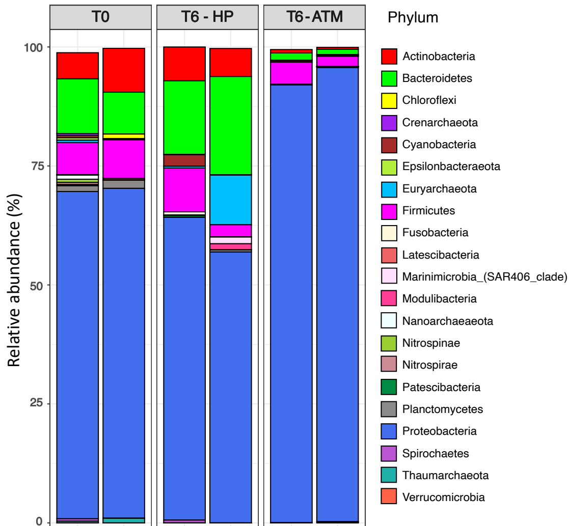
Figure 4-3 Relative abundance (%) of the most actively transcribed prokaryotes (>0.01% in average) initially (T0) and after 6 days of incubation under increasing pressure (T6-HP) and atmospheric pressure (T6-ATM) conditions.
