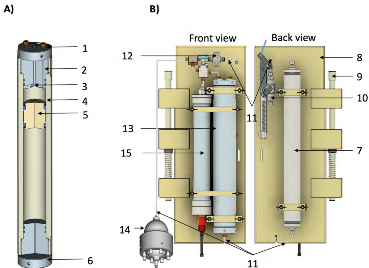
Figure 2-1 (A) Cross section of the Titanium TA6V 500mL High Pressure Bottle (HPBs). (B) Schematic drawing of the front and back views of the High-Pressure Sample Unit (HPSU). 1. Top end-cap devoted to oxygen measurement; 2. 1/8" (3.2mm O.D.) Inlet flowthrough; 3. Sapphire window; 4. Main core; 5. PEEK floating-piston with lip seal; 6. Bottom end-cap. In the part, above floating-piston seawater sample is in contact with sapphire window (see details in the text). The part below the floating-piston contains sterile milliQ water which serve as hydraulic brakes when passing through the thin catheter into the exhaust tank (7); 8. Polypropylene main frame; 9. Push rod for attachment to a rosette system. When the (10) inlet-valve is opened by magnetically activated lanyard release, the seawater enters the hydraulic circuit through a 1/8" (3.2mm O.D.) stainless-steel tube (11), via one check valve (12), to fill in the HPB (13), the pressure accumulator (14), and the aero-hydraulic pressure sensor (15).
