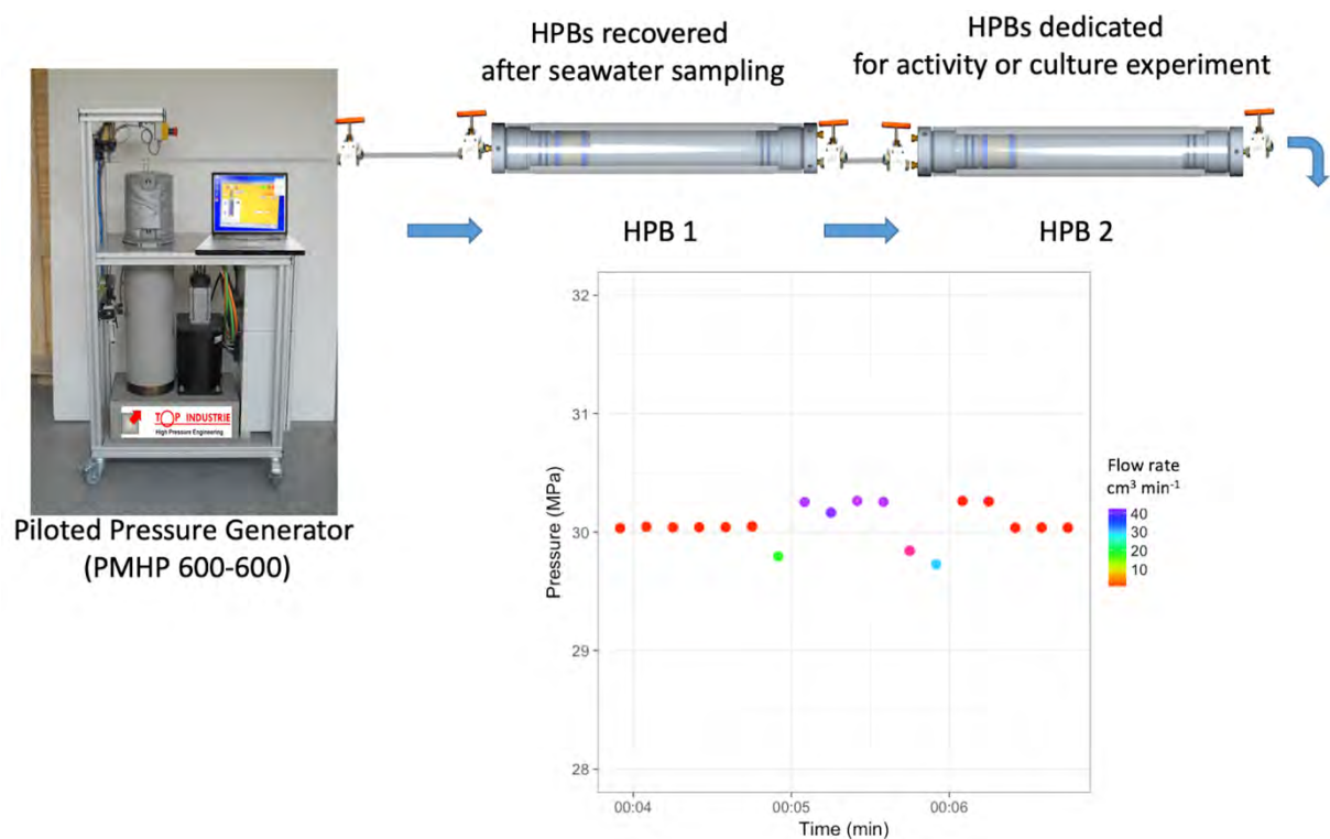
Figure 2-3 Transfer in equi-pressure mode. After sampling HPBs dedicated to sample (HPB 1) are connected at bottom end-cap to piloted pressure generator (PMHP 600-600) and at top end-cap to HPB dedicated to activity measurement or culture experiments (HPB 2), previously pressurized at the working pressure. In the example, the PMHP 600-600 and the HPB2 are preconditioned to 30 MPa, the same hydrostatic pressure of the 3000 m-depth sample of the HPB1. During the transfer, the PMHP 600-600 prevents pressure loss by adding milliQ water at the working pressure into the lower part of HPB 1, the sample being isolated by the floating piston. The equivalent volume of the seawater sample enters HPB 2, which is managed by a handle valve at the bottom end-cap. Data is recorded during transfer in equi-pressure mode with a time-step of 10 s. The transfer takes about 2 minutes for a volume of 40 mL with an accuracy of less than 0.5 MPa.
