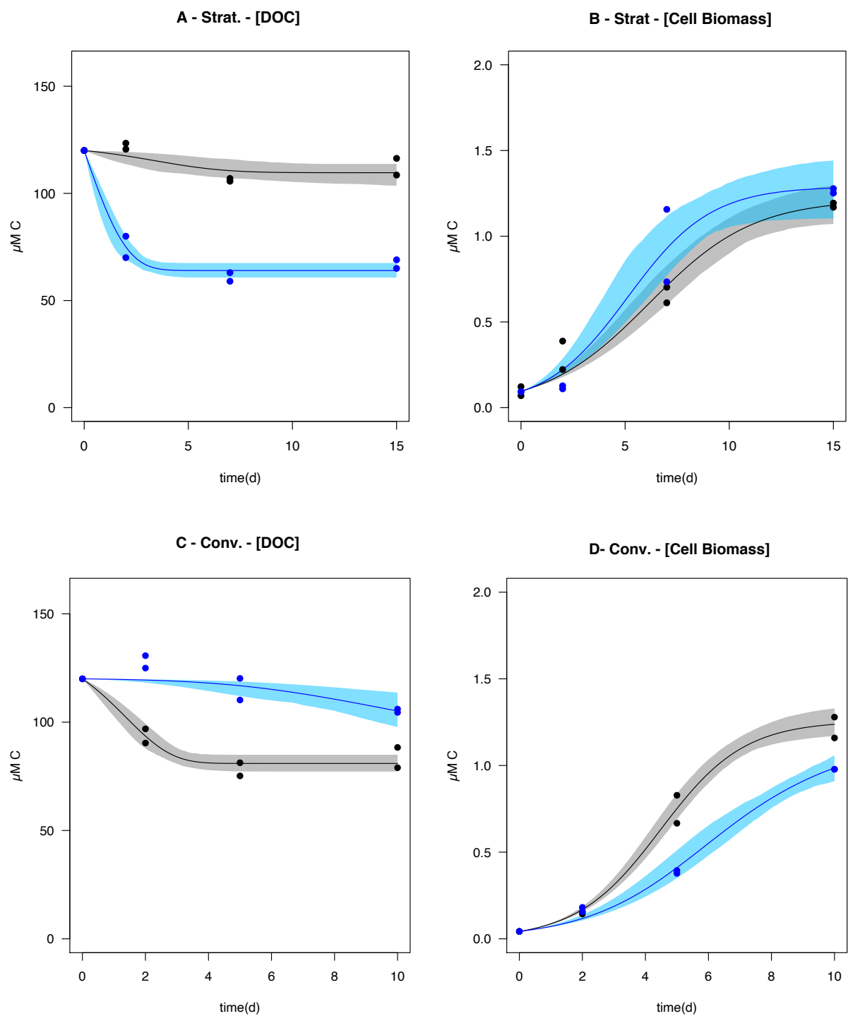
Figure 3-2 Changes in DOC concentrations (A, C), cell biomass concentrations (B, D) in \mu\text{M C} over time (in days) during stratified period (Strat.) and deep-water mass convection period (Conv.). Blue and black dots are observations respectively for HP and DEC incubations. Blue and black lines are predicted data by model and blue and grey variability bands are 95% confident intervals, respectively for HP and DEC incubations.
