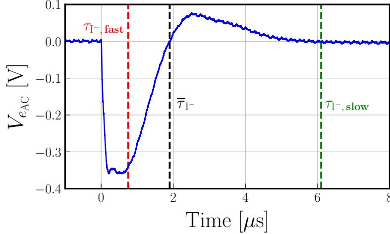
Figure 3.32: Photodetachment signal obtained for a pressure of 1.5 mTorr and a discharge power of 100 W at z = 3 cm from the antenna. The negative ions characteristic times ( \tau_{I^-} , fast , \bar{\tau}_{I^-} and \tau_{I^-} , slow ) are indicated by vertical dashed lines.
