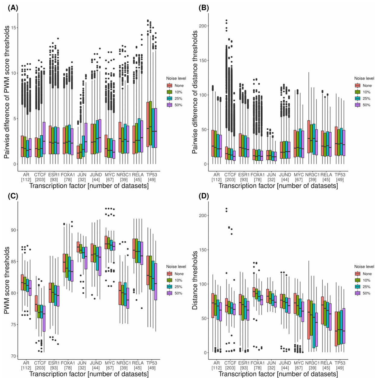
Supplementary Figure S7: Assessment of the robustness to noise for ChIP-eat to define enrichment zones. Boxplots of the pairwise differences for the thresholds on PWM scores (A) and distances to peak summits (B) between ChIP-seq data sets for the same TF are provided in the upper panels. Boxplot of the absolute threshold values for the PWM scores (C) and distances to the peak summits (D) are provided in the lower panels. In all panels, results from the original sets of peaks are provided in red. We added noise (random sequences) to the initial set of ChIP-seq peaks for each dataset (see Materials and Methods) to test the variability of the thresholds. Three levels of noise were assessed: 10% (green), 25% (blue), and 50% (violet).
