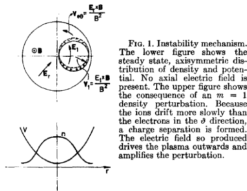
Figure 3.6.: Mechanism of neutral drag instability. Source[Hoh63a]
