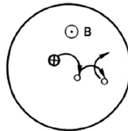
Figure 4.3.: Diffusion of gyrating particles by collisions with neutral atoms. Source[Che16]
