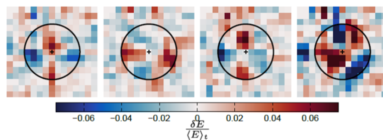
Figure 2.9.: Evolution of the emissivity variation \delta E for a m = 2 rotating mode. Each image is separated by 45 \mu\text{s} and the period of the mode of about 195 \mu\text{s} . Values are normalized to the average emissivity at the center. Source [Dav17]
