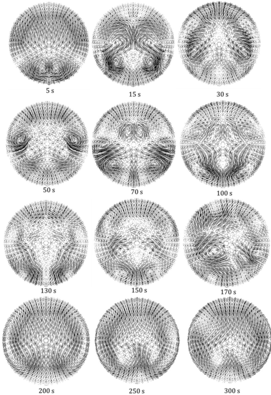
Figure 32. – Velocity profile in 3D at the downstream of elbow from stagnant state over time by TrioCFD.
